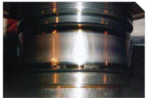
FIGURE 5 - Inner race of same NU326 greased bearing after disassembly.
