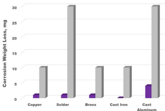
ASTM D1384 Coolant Corrosion Test
