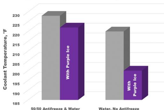
Dyno Testing Coolant Temperature
